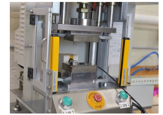
LPMS Overmolding Machines
